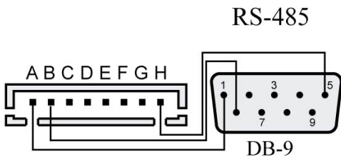
J1 connect to TCP/IP or RS485 converter
