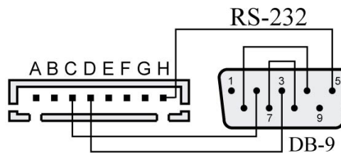
J1 connect to DB9(PC)
